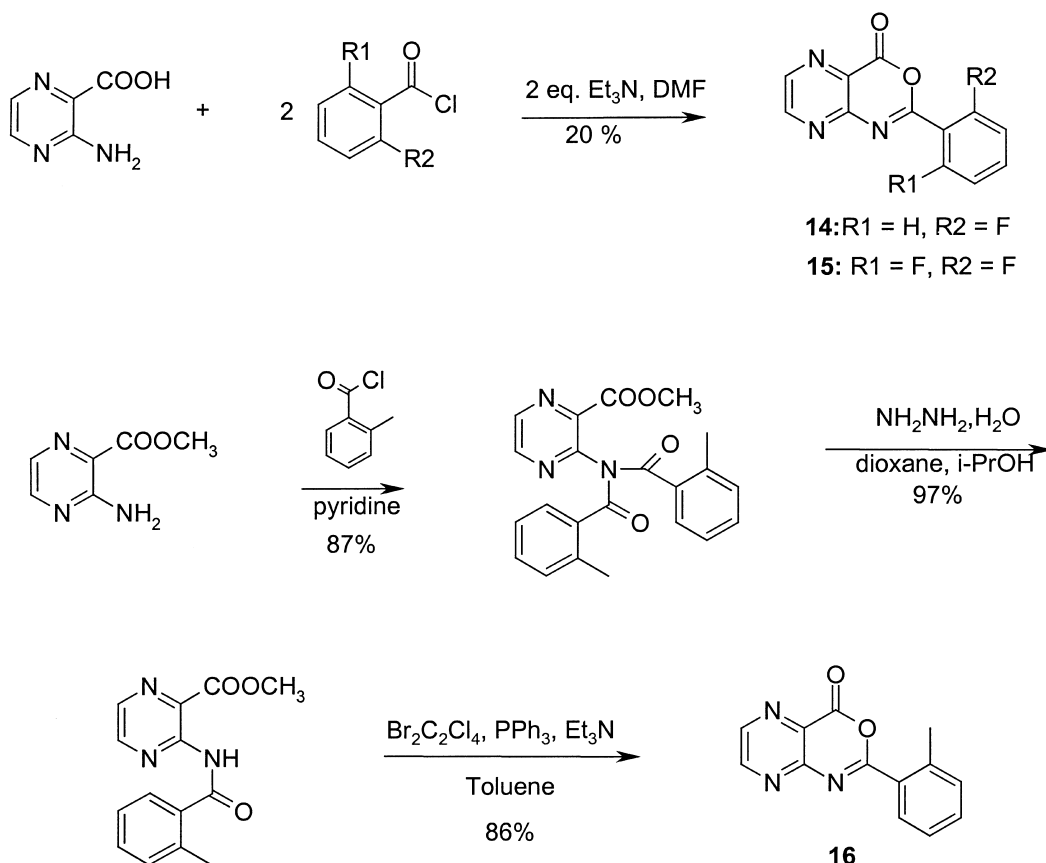
Scheme 2. Reaction pathway to pyrazino[2,3-d][1,3]oxazin-4-ones 14–16 .
