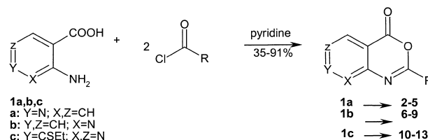
Scheme 1. Reaction pathway for pyridines and pyrimidines. (Compound: R): 2 , 7 : 2,6-F 2 Ph; 3 , 6 , 10 : 2-FPh; 4 , 8 : 2-thienyl; 5 , 9 : 2-furanyl; 11 : 2-NO 2 Ph; 12 : 2-MePh; 13 : 2-ClPh.
