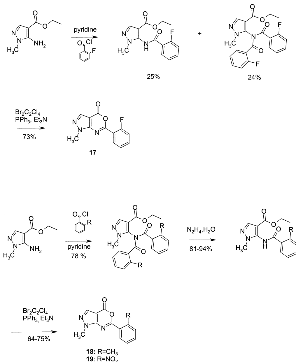
Scheme 3. Synthetic pathway to pyrazolo[2,3- d ][1,3]oxazin-4-ones 17 – 19 .
