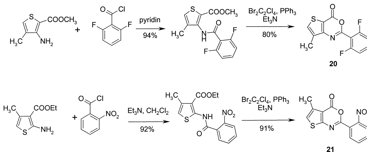
Scheme 4. Synthetic pathway to thieno[3,2-d][1,3]- and thieno[2,3-d][1,3]-oxazin-4-ones 20 and 21 .
